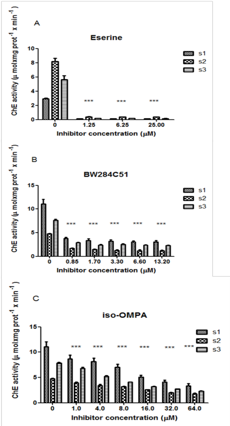
Figure 1: Effect of specific inhibitors of cholinesterase activity. Results showed three placenta samples (s1, s2 and s3) and they are expressed in \mu\text{mol} of substrate hydrolyzed \text{mg protein}^{-1} \text{ min}^{-1} . ANOVA: *** p < 0.0001
