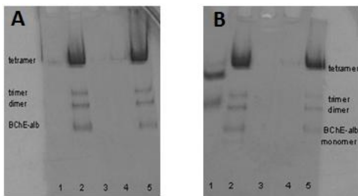
Figure 3: Non-denaturing gel stained for activity with BSCh (A) and ASCh(B).
